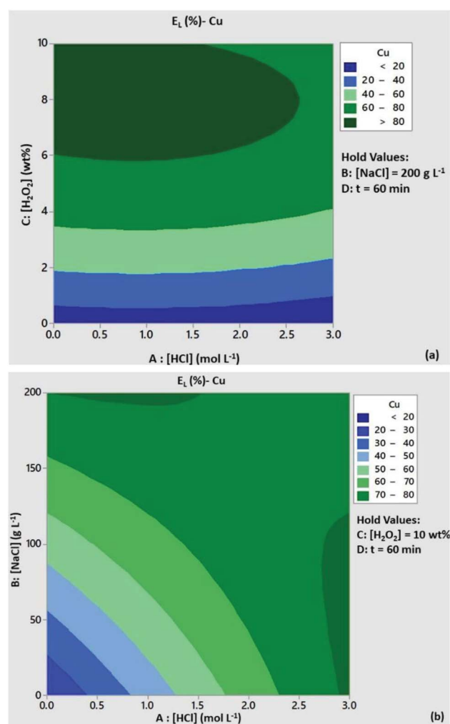
Fig. 2 Contour plots of Cu leaching efficiency as a function of (a) [\text{HCl}]/[\text{H}_2\text{O}_2] and (b) [\text{HCl}]/[\text{NaCl}] . Conditions: L/S = 10 \text{ mL g}^{-1} , T = 80 \text{ }^\circ\text{C} , t = 60 \text{ min} and (a) [\text{NaCl}] = 200 \text{ g L}^{-1} , (b) [\text{H}_2\text{O}_2] = 10 \text{ wt}\% .
